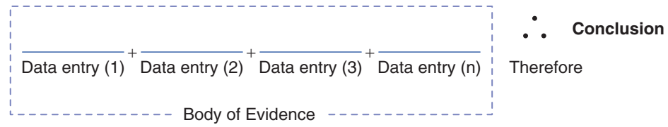
Figure 4.7 Joint Reasoning
