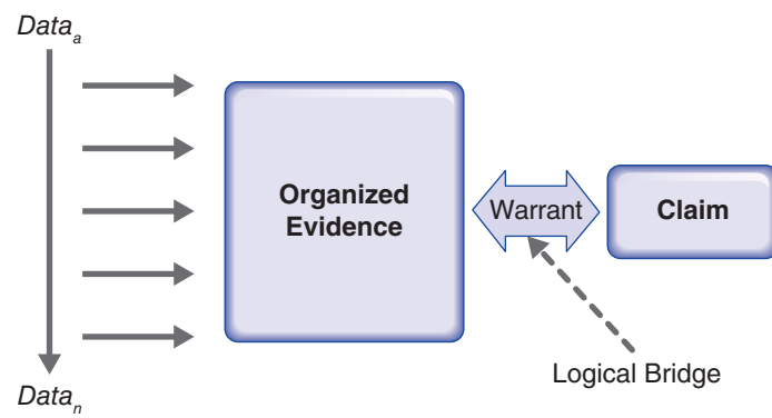
Figure 2.4 The Simple Argument: The Logic of the Argument
